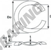
Split Wave Spring Washers
