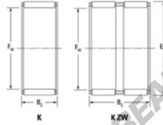
123 Bearing Boundary dimensions for needle roller and cage assemblies
